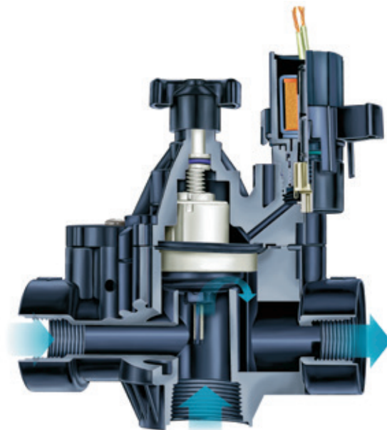
PGA Cutaway
