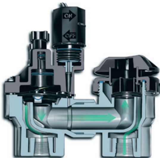
ASVF Cutaway
